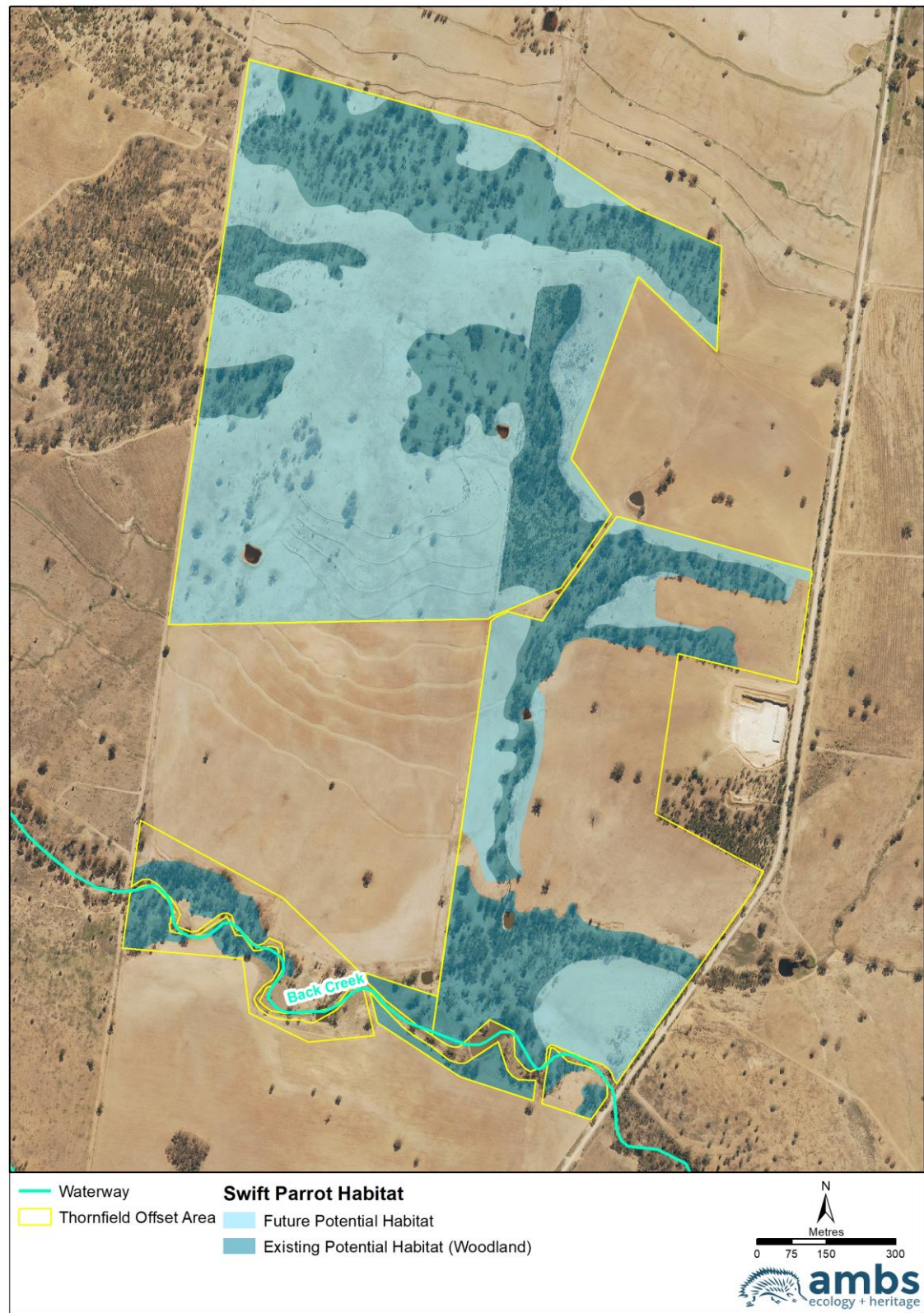
Figure 3.2: Swift Parrot Habitat and Future Potential Habitat in the Thornfield Offset Area
